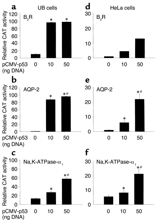
Figure 3 Exogenous wild-type p53 transactivates the RFG promoters. UB or HeLa cells were cotransfected with 0, 10, or 50 ng of pCMV-p53 plasmid DNA and 1.2 \mu g each of promoter-reporter constructs for rat B 2 R (a and d), mouse AQP-2 (b and e), and human Na,K-ATPase- \alpha_1 (c and f). pSV-lacZ (0.5 \mu g) was cotransfected to measure transfection efficiency. Cellular extracts were harvested 24 hours after transfection and assayed for CAT activity (percent acetylation). The results are mean \pm SE of three experiments performed in duplicate. * P < 0.001 versus 0 ng p53; # P < 0.05 versus 10 ng p53.
